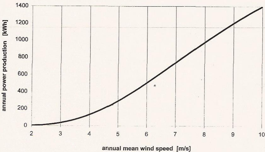
Annual Power Production
