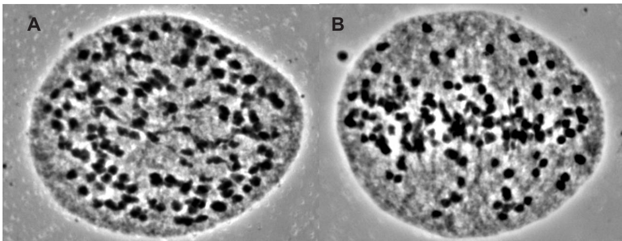
Figure 2: Meiotic chromosome squashes from \times Cystocarpium rosamianum . A, Cell at late prophase I, showing approximately 140 chromosomes, predominantly univalents but some loosely paired bivalents. B, Cell at metaphase I/early anaphase I, in which the bivalents are pulled to the metaphase plate while the univalents remain scattered throughout the cytoplasm.
