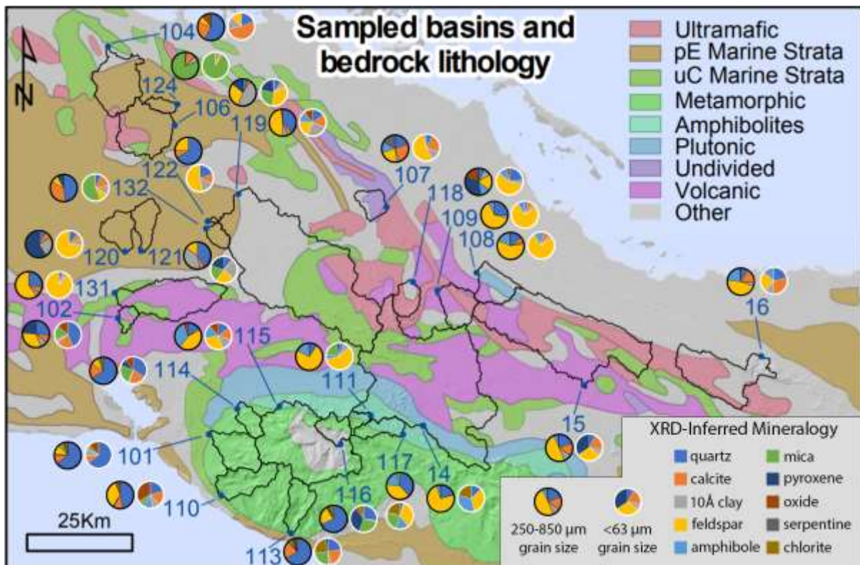
Fig. 3, Map showing sampling locations and watershed area, underlying lithology, and XRD-derived mineralogy data in two grain sizes. Modified from Bierman et al., (2020).
