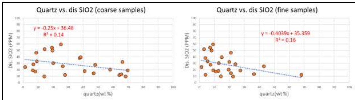
Fig. 7, Regressions between dissolved SiO 2 in stream water (Bierman et al., 2020) measured in the field and mineralogy in two grain sizes (<63 μm and 250-850 μm) (this study) measured using XRD.
