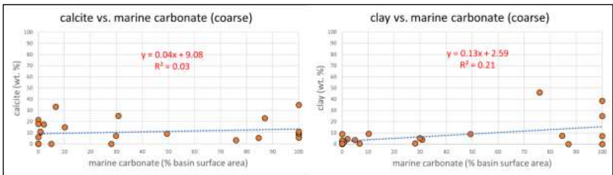
Fig. 5 , regressions between marine carbonate lithologic units (Case and Holcombe, 1980) and mineralogy (this study) measured using XRD.
