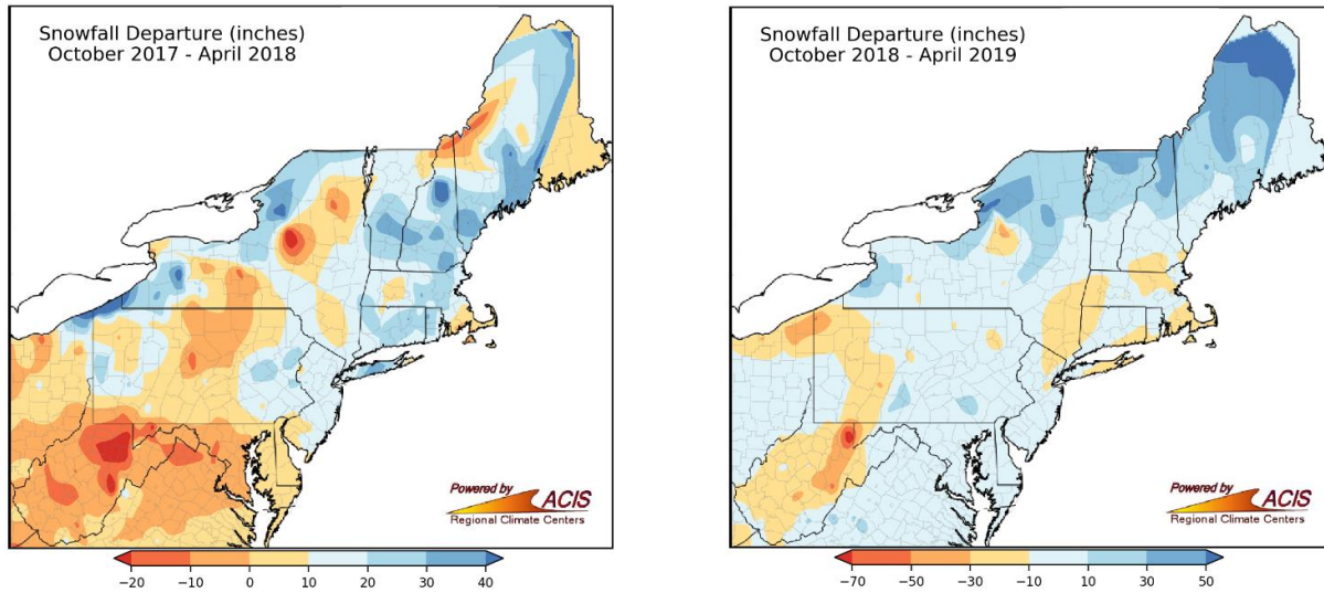
Figure 18. Regional snowfall departure from long-term normal for the winters at the beginning and end of 2018. The winter going into 2019 had more than average snow accumulation across the region, while the winter at the beginning of 2018 was variable across the region. Note the different scales in the two maps. Figure credit: NOAA, Northeast Regional Climate Center at Cornell University.
