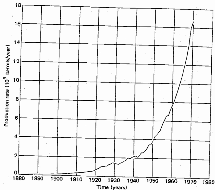
Figure 5.2 World production of crude oil (Hubbert, 1974a, fig. 5).
