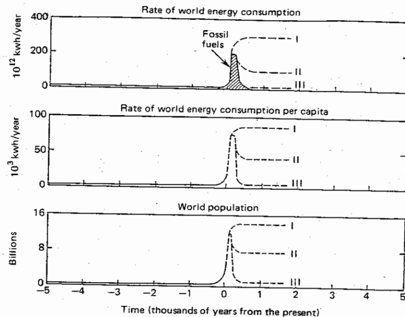
Figure 5.11 Human affairs in historical perspective from 5,000 years in the past to 5,000 years in the future (after Hubbert, 1962, fig. 61).
