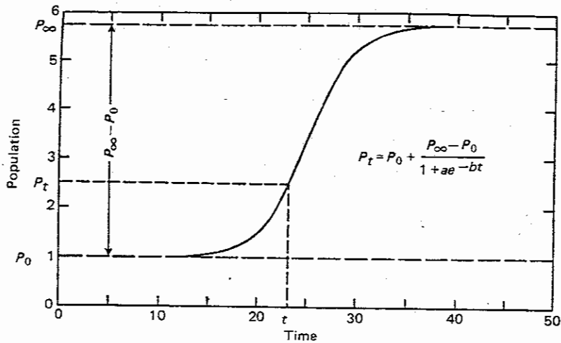
Figure 5.3 Logistic curve of population growth.
