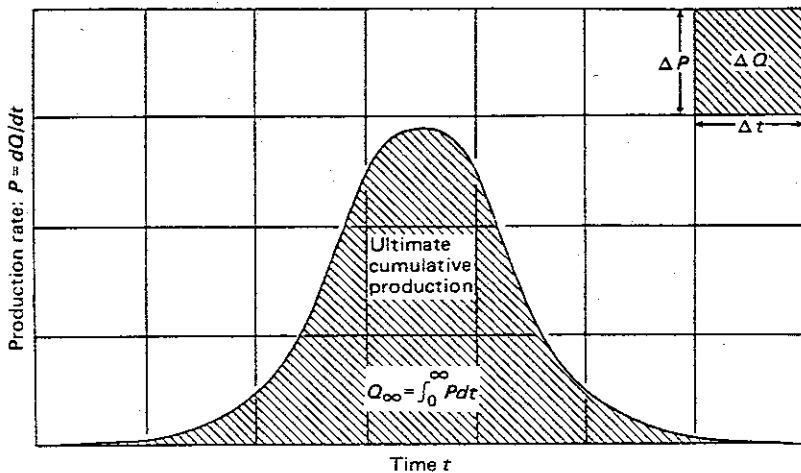
Figure 5.6 Mathematical properties of complete-cycle curve of production of an exhaustible resource (Hubbert, 1974a, fig. 18).
