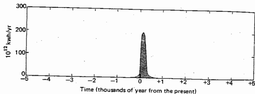
Figure 5.10 Epoch of fossil fuel exploitation in human history during the period from 5,000 years ago to 5,000 years in the future (Hubbert, 1974a, fig. 69).
