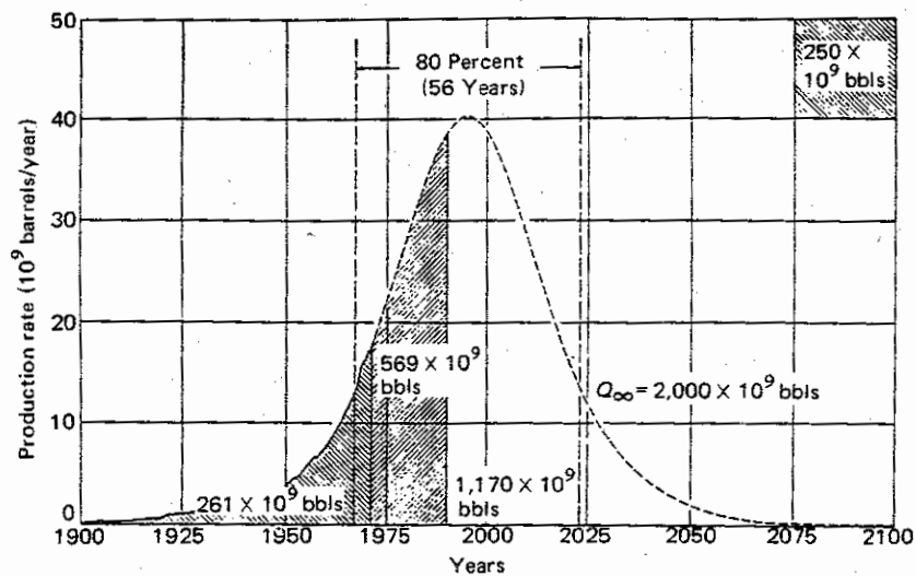
Figure 5.8 Complete-cycle curve for world crude oil production (Hubbert, 1974a, fig. 68).
