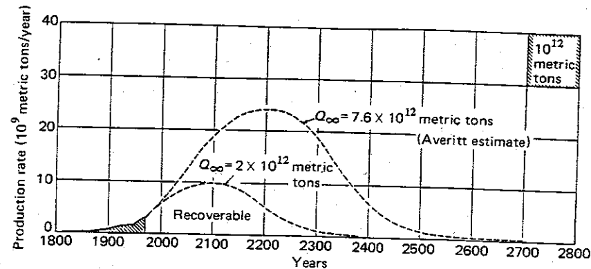
Figure 5.7 Complete-cycle curves of world coal production for higher figure of 7.6 \times 10^{12} and lower figure of 2 \times 10^{12} metric tons for ultimate production (Hubbert, 1974a, fig. 21).
